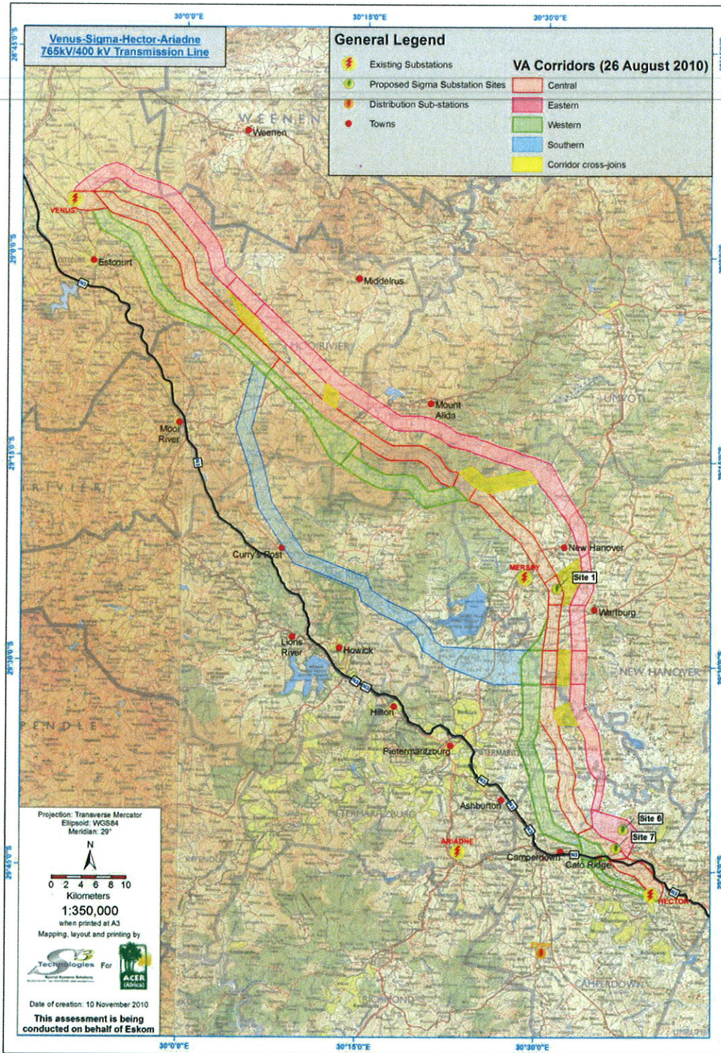
Figure 2 Proposed VSHA Transmission Line Corridors
